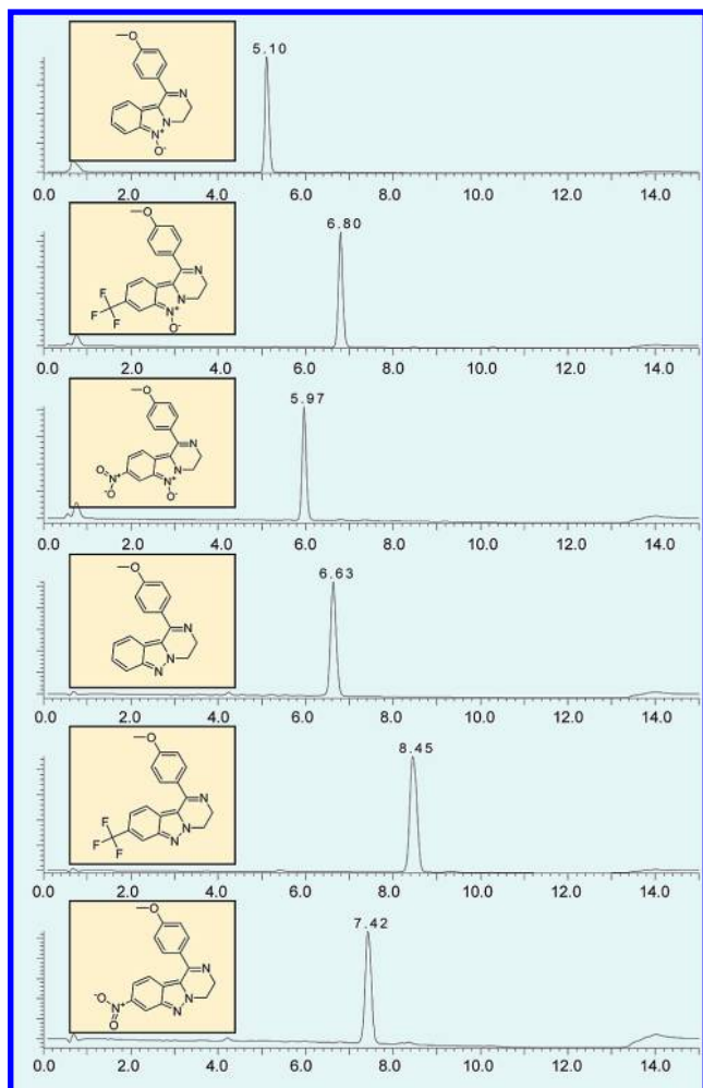
Figure 2. LC traces of crude compounds 7 and 8.
